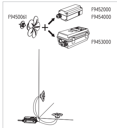
Junction box without remote housing, for wall/ground fittings with remote power
