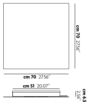
Wall / Ceiling Large square AP1-PL1
