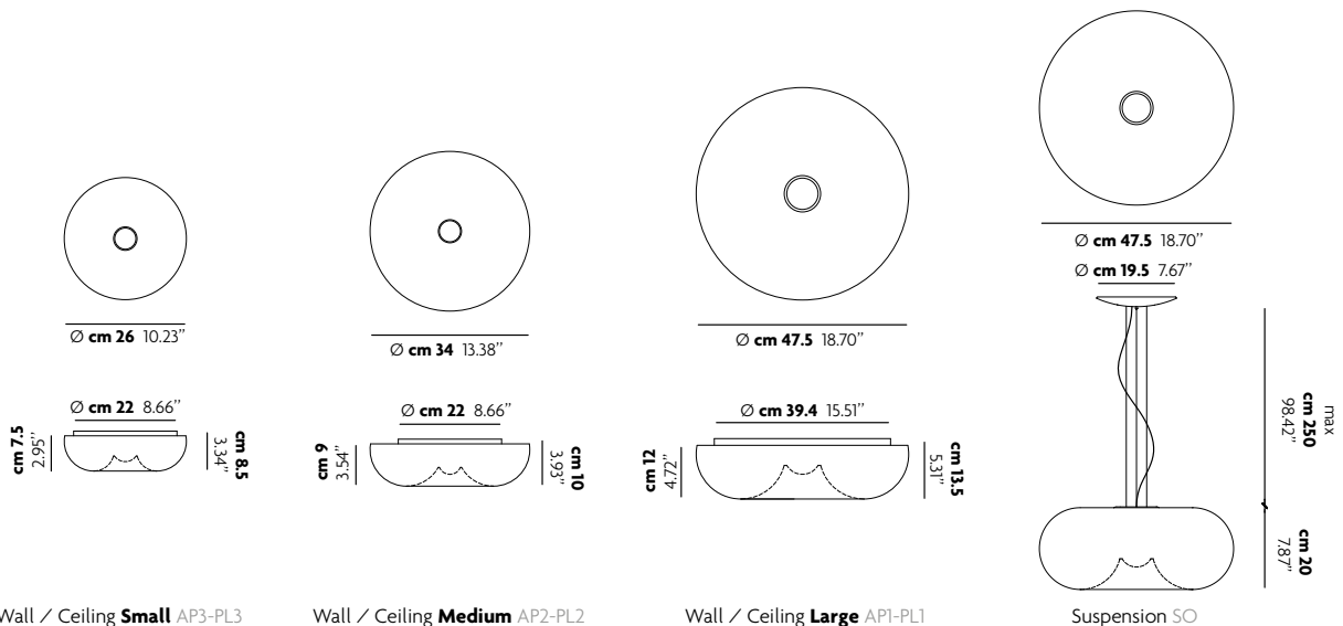
Wall / Ceiling Small AP3-PL3
