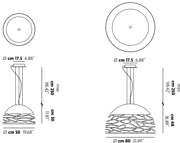
Suspension Medium dome SO1
