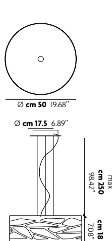
Suspension Medium cylinder SO1
