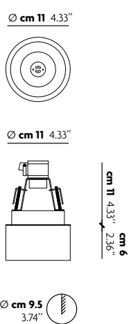
Recessed Campy INC
