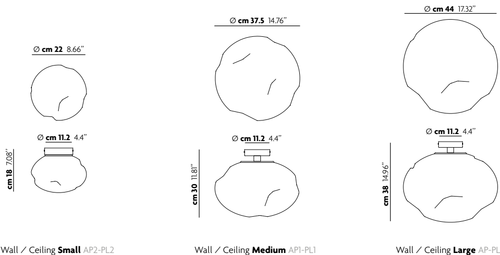
Wall / Ceiling Small AP2-PL2
