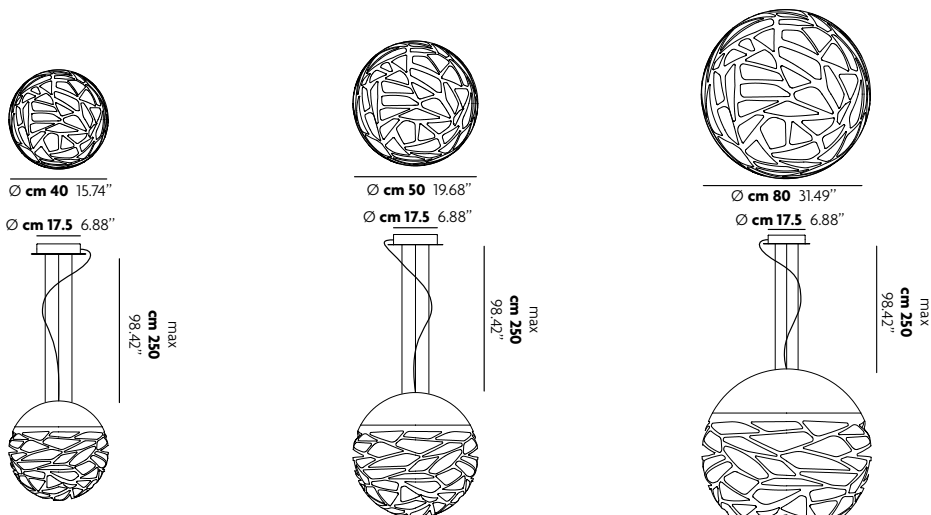
Suspension Small Sphere SO2
