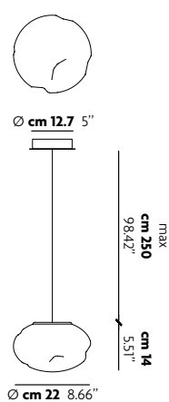
Suspension Small SO2
