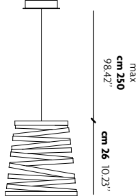
Suspension Small SO
