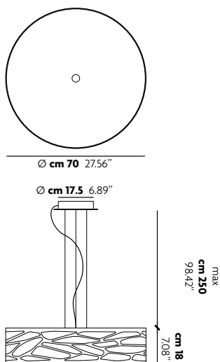
Suspension Large cylinder SO
