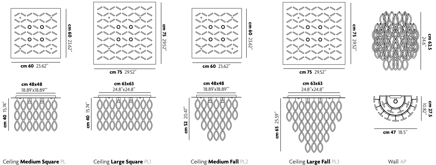
Ceiling Medium Square PL
