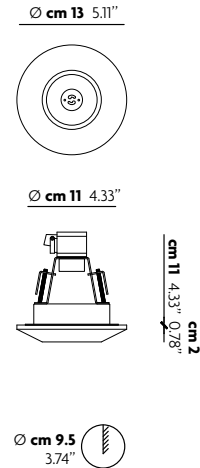
Recessed Twin INC
