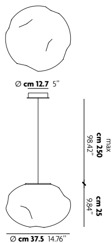
Suspension Medium SO1
