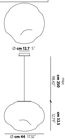
Suspension Large SO
